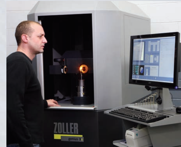
A 5-axis Zoller Automatic Measuring Machine precisely checks to validate that tools meet exact specifications.
